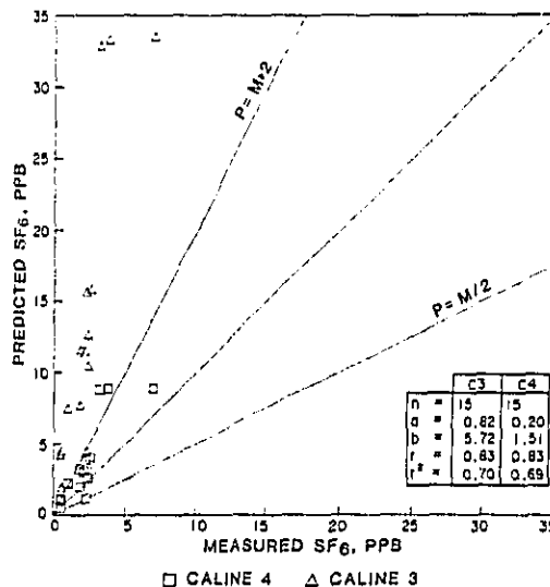
FIGURE 3 Zone 1 predicted versus measured SF 6 levels.
