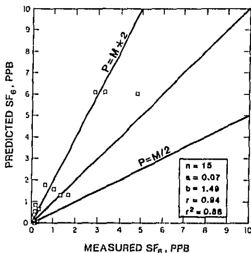
FIGURE 4 Zone 2 predicted versus measured SF 6 levels.
