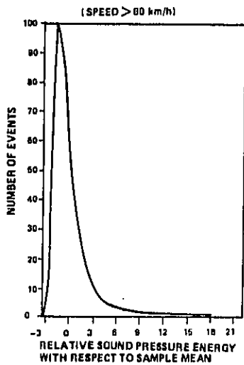
FIGURE 12 Heavy-truck noise distribution: energy.
