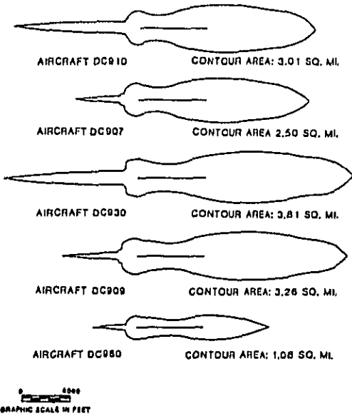
FIGURE 4 DC-9 aircraft noise contours.
