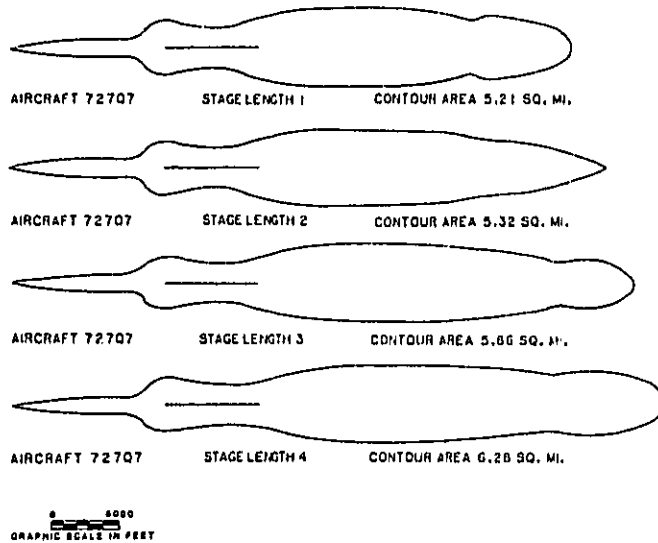
FIGURE 11 B727 stage length comparison.
