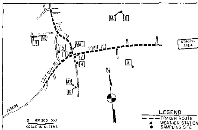
FIGURE 1 Tracer study sampling site location map.
