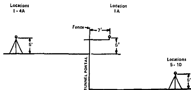
FIGURE 5 Instrument set-up.
