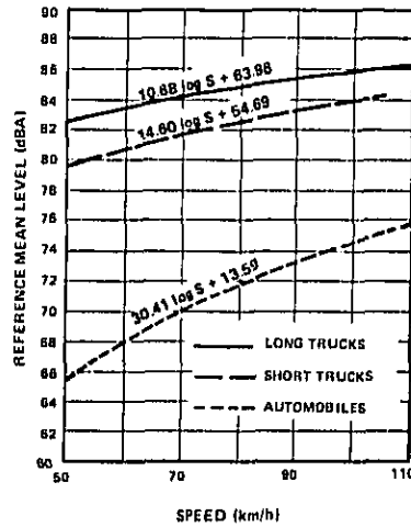
FIGURE 8 Emission levels of Ontario vehicles classified according to short trucks versus long trucks.
