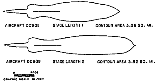
FIGURE 10 DC-9 stage length comparison.
