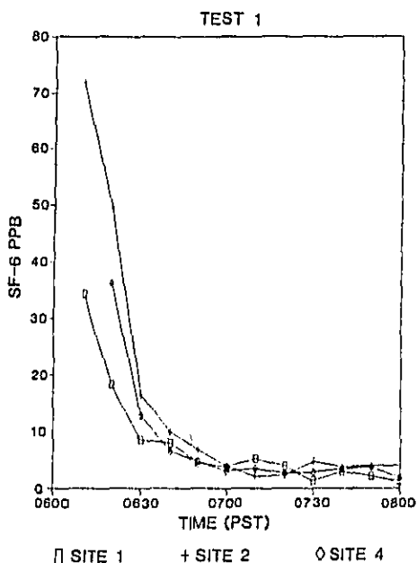
FIGURE 2 Test 1: 10-min integrated samples.
