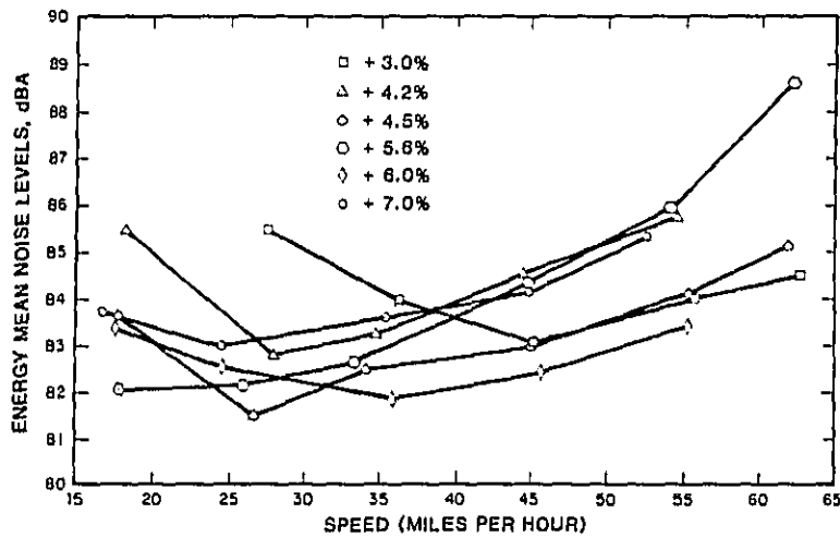
FIGURE 10 Plots by means of 10-mph speed classes (speed versus L_{90} ).
