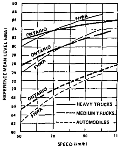
FIGURE 9 Comparison of Figure 7 emission levels with original FHWA levels (1).
