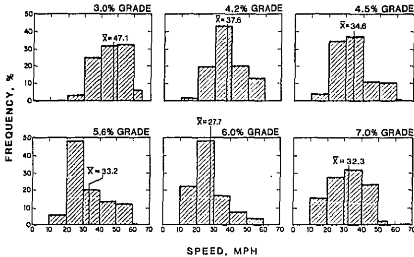
FIGURE 14 Speed distributions by grade.
