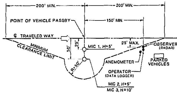
FIGURE 3 Typical site layout and microphone locations.
