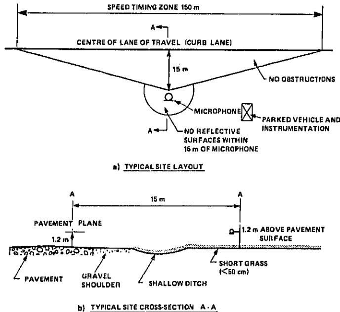
FIGURE 1 Typical layout of roadside measurements.
