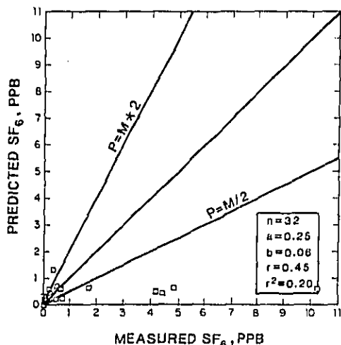
FIGURE 5 Zone 3 predicted versus measured SF 6 levels.
