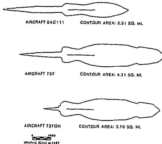
FIGURE 5 BAC111 and B727 aircraft noise contours.
