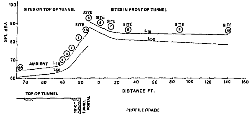
FIGURE 6 L_{10} and L_{50} sound level versus distance.
