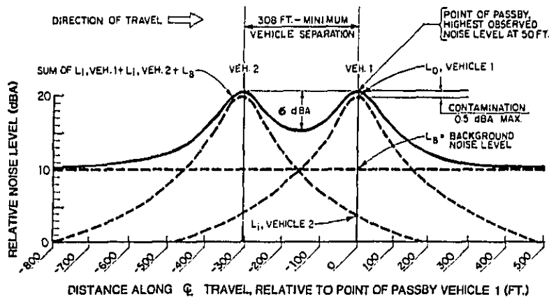
FIGURE 4 Minimum separation between two heavy trucks.
